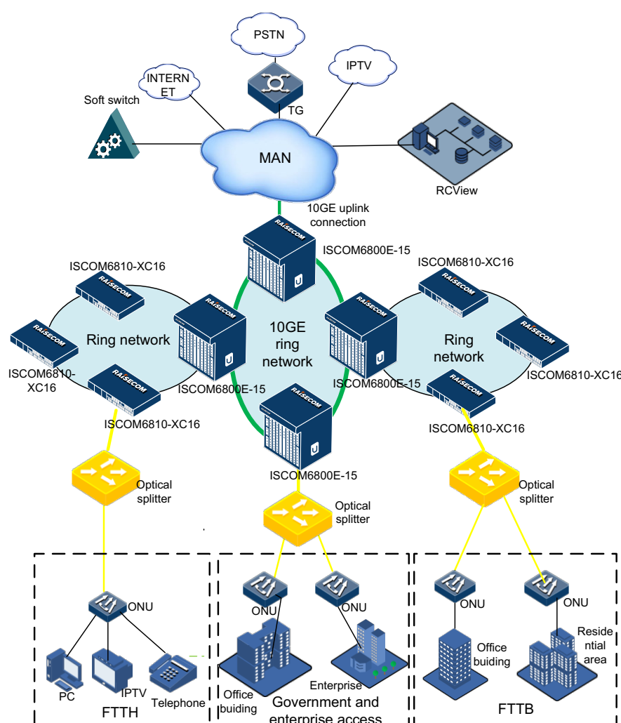
Figure 1 Ring network with the ISCOM6810-XC16 and ISCOM6800E-15
