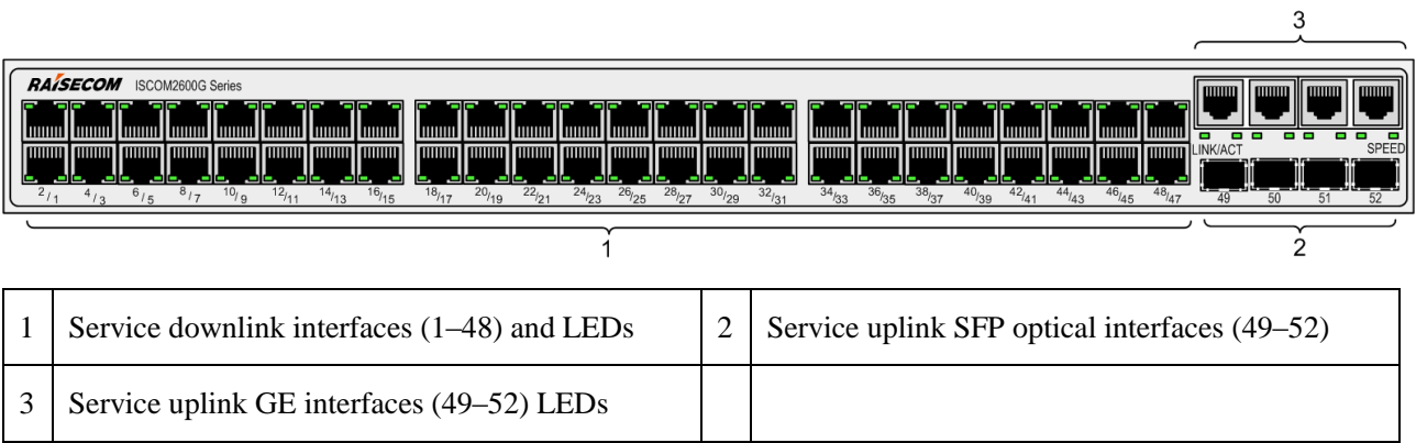
Figure 3-13 Front panel of the ISCOM2648G-4GE-RPS-AC
