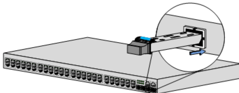
Figure 4-8 Inserting SFP optical module
