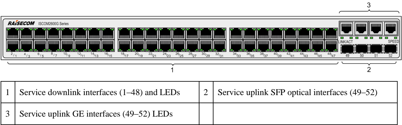
Figure 3-12 Front panel of the ISCOM2648G-4GE-AC/DC
