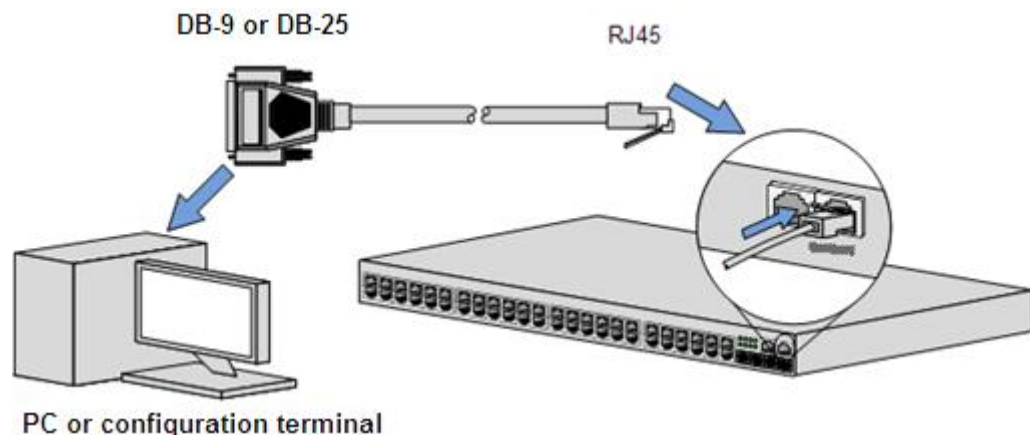
Figure 4-14 Connecting RJ45 Console cable
