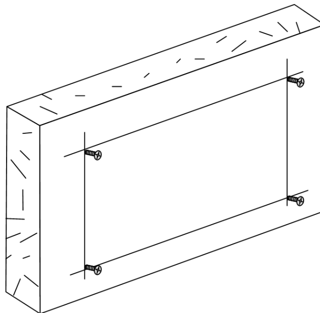
Figure 4-6 Installing screws
