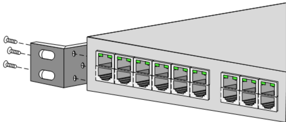
Figure 4-1 Installing brackets
