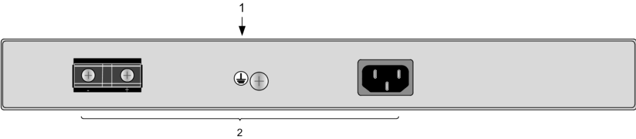
Figure 3-33 Rear panel of the ISCOM2648G-4C-AC_DC
