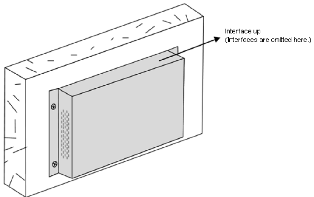
Figure 4-7 Wall-mount installation
