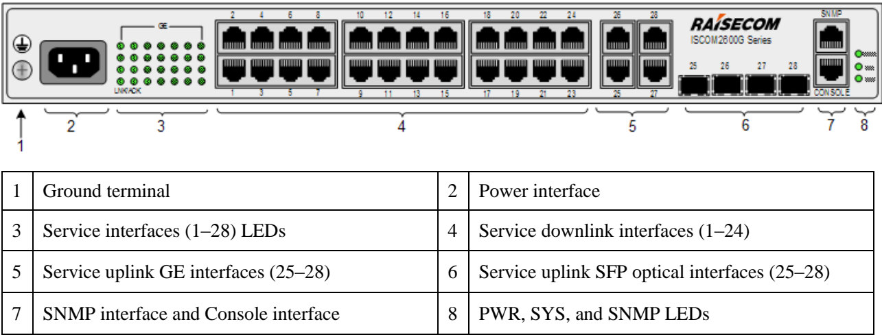
Figure 3-6 Front panel of ISCOM2624G-4GE-AC
