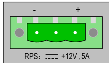
Figure 3-37 ISCOM2648G-4GE-RPS-AC power interface
