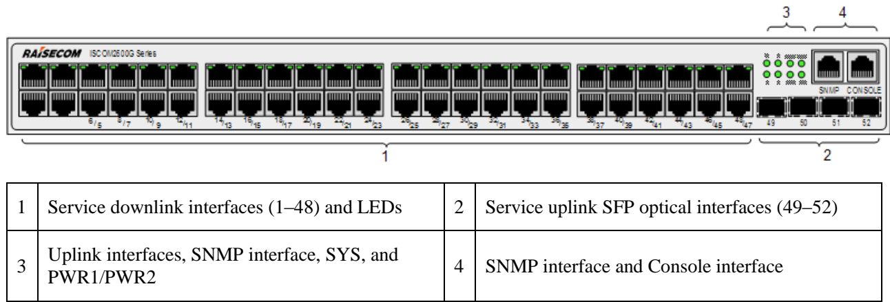
Figure 3-15 Front panel of the ISCOM2648G-4C-AC/DC/D
