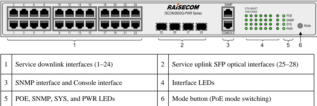
Figure 3-5 Front panel of ISCOM2624G-4C-PWR-AC/DC
