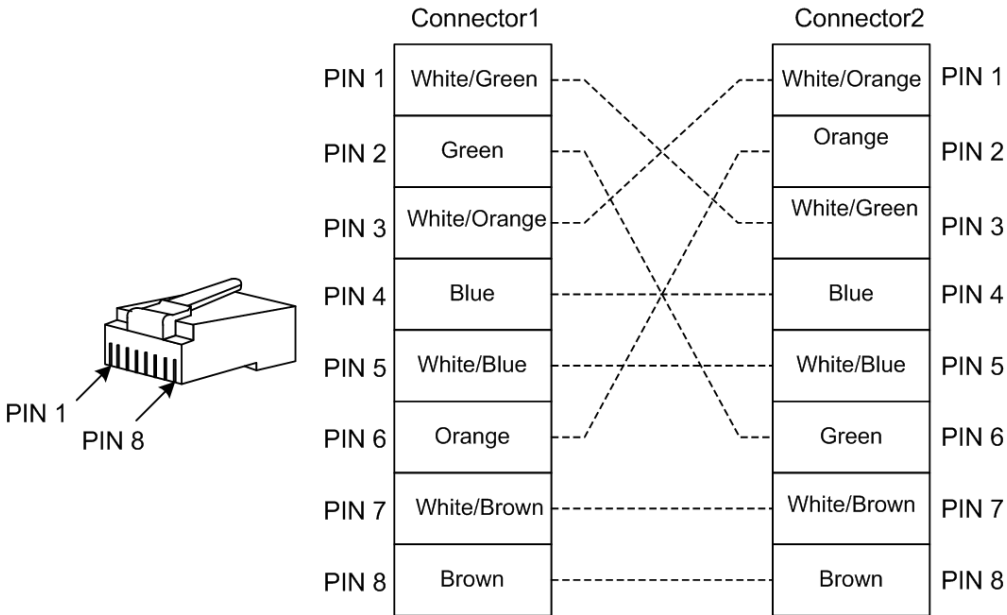
Figure 6-4 Wiring of 100 Mbit/s crossover cable
