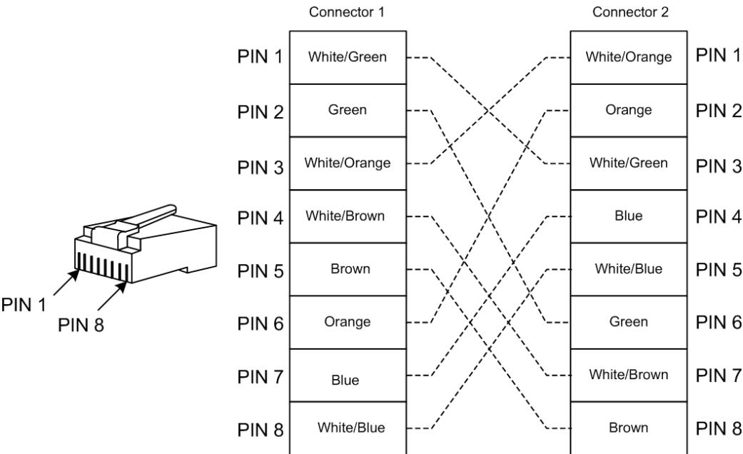
Figure 6-5 Wiring of 1000 Mbit/s crossover cable
