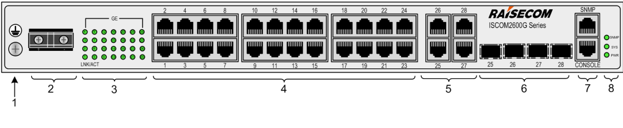
Figure 3-7 Front panel of ISCOM2624G-4GE-DC
