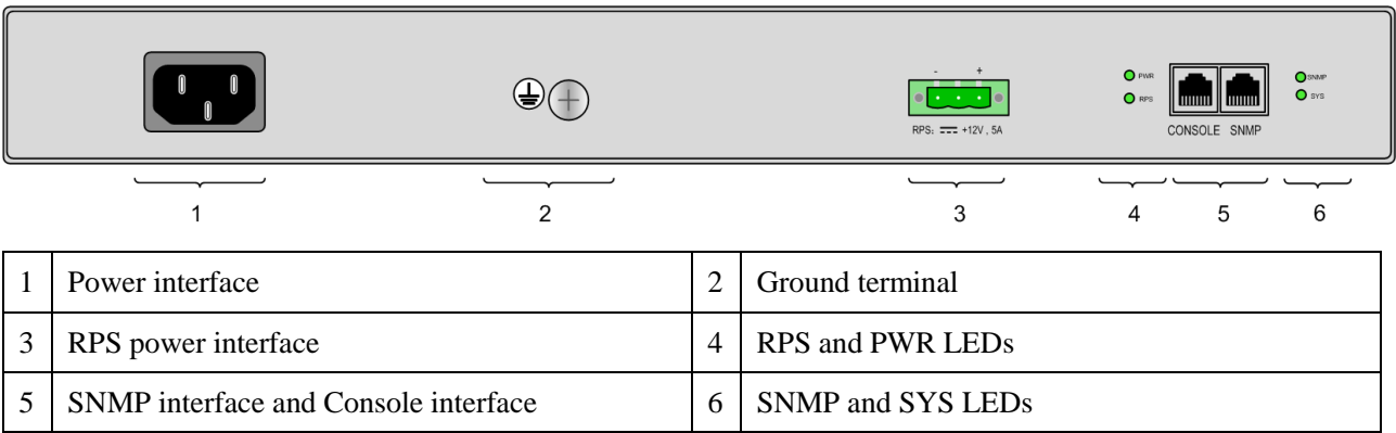
Figure 3-28 Rear panel of the ISCOM2648G-4GE-RPS-AC
