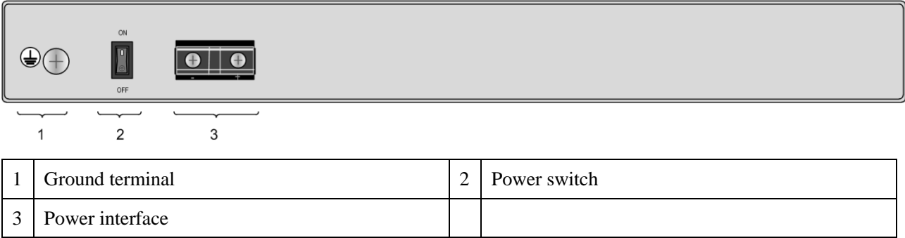
Figure 3-23 Rear panel of ISCOM2624G-4GE-PWR-DC
